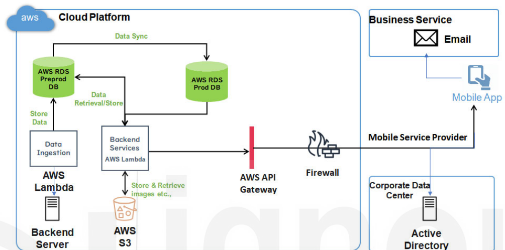
Figure 1 Mobile computing system that uses services distributed across cloud and data centre.
